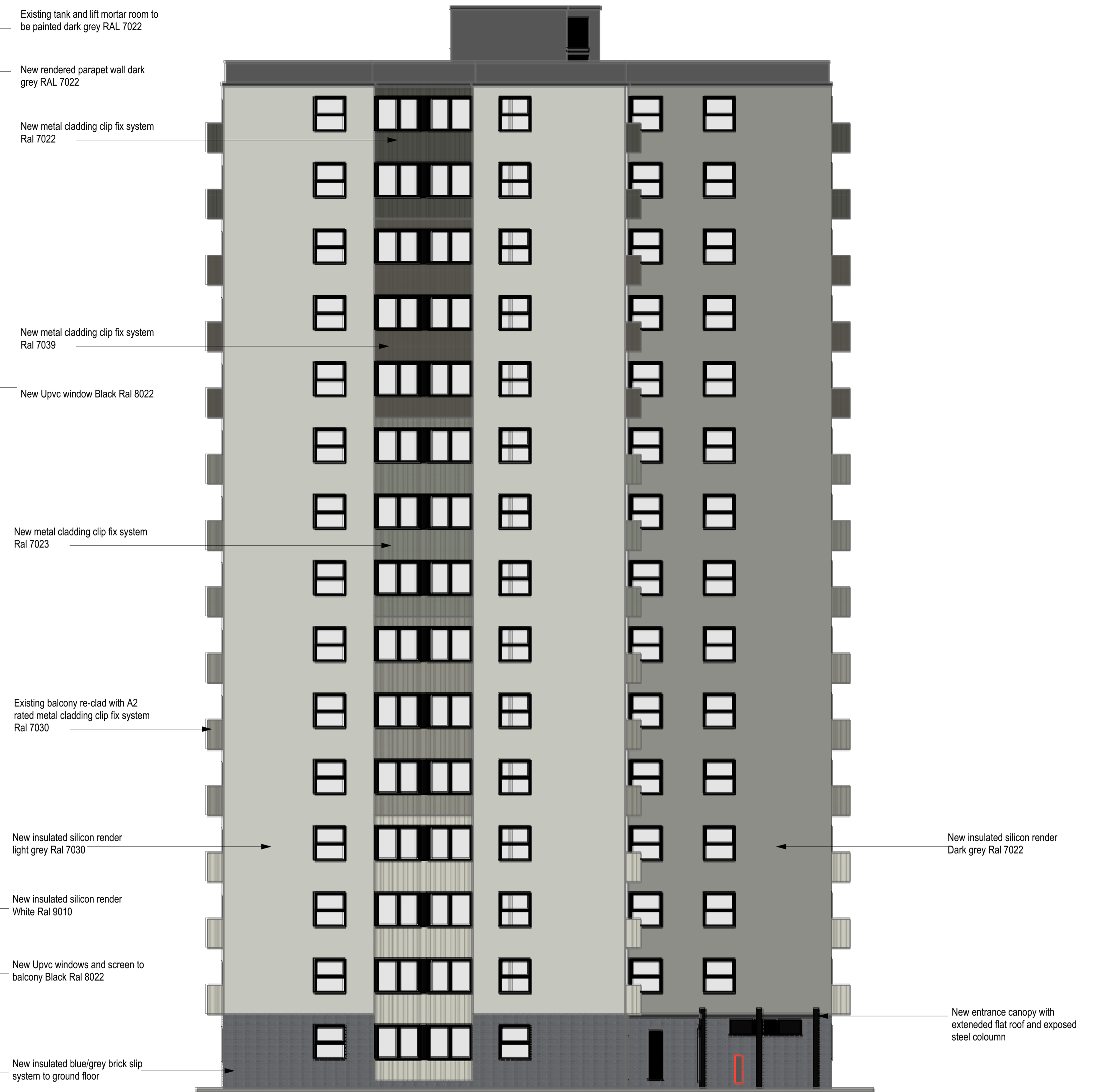
WHITE FRIAR COURT SIDE ELEVATION
