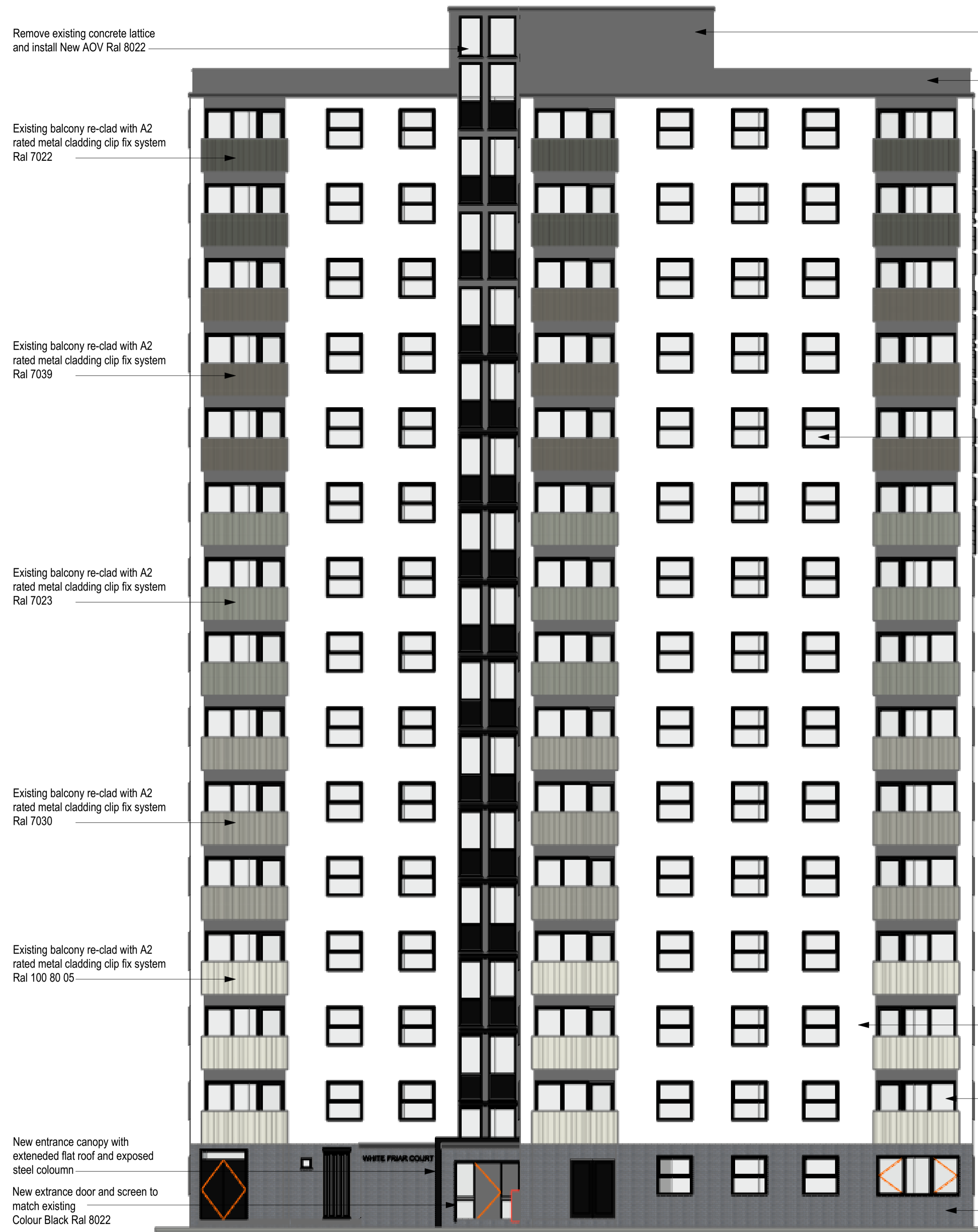
WHITE FRIAR COURT FRONT ELEVATION
