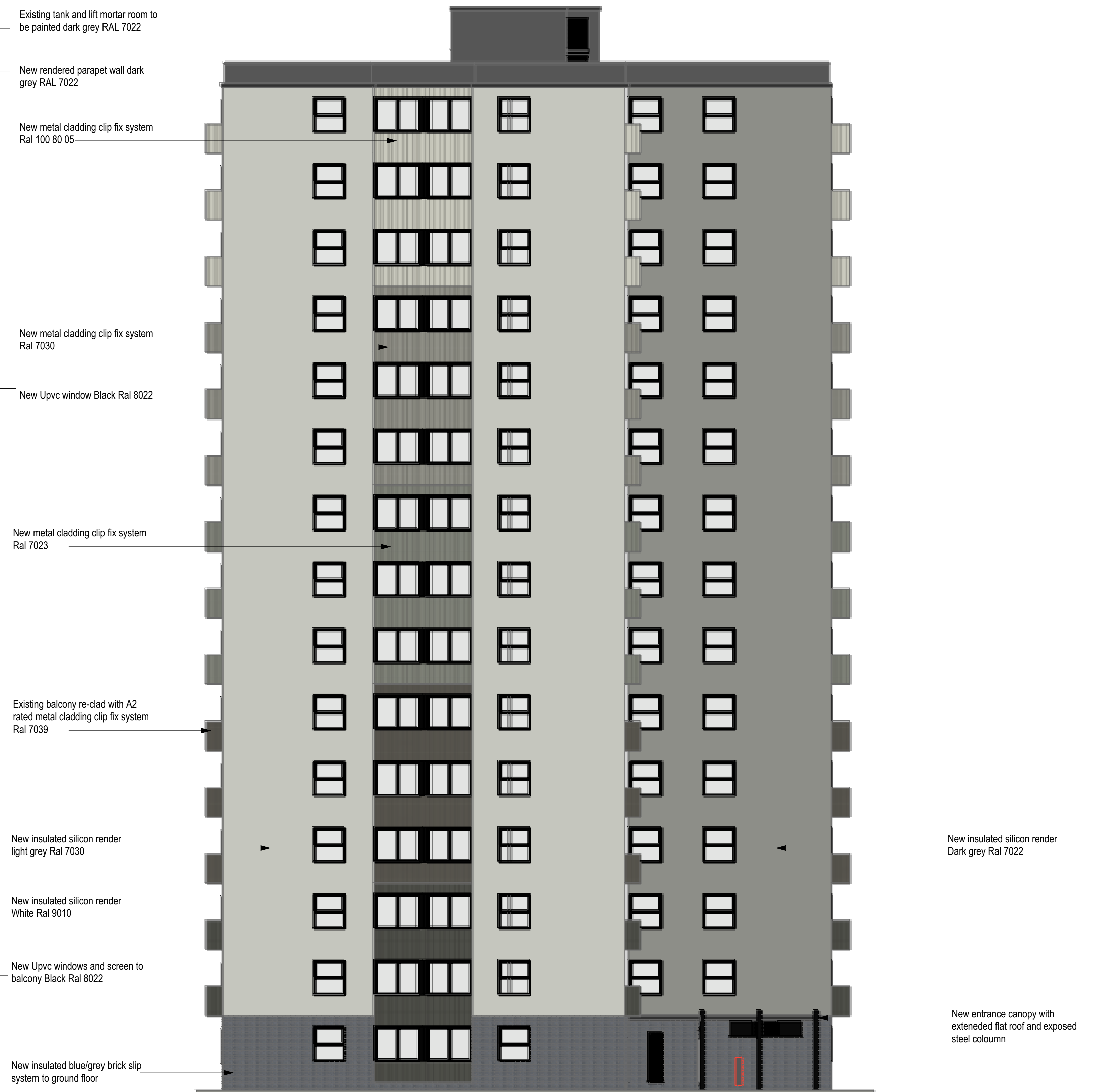
GREY FRIAR COURT SIDE ELEVATION
