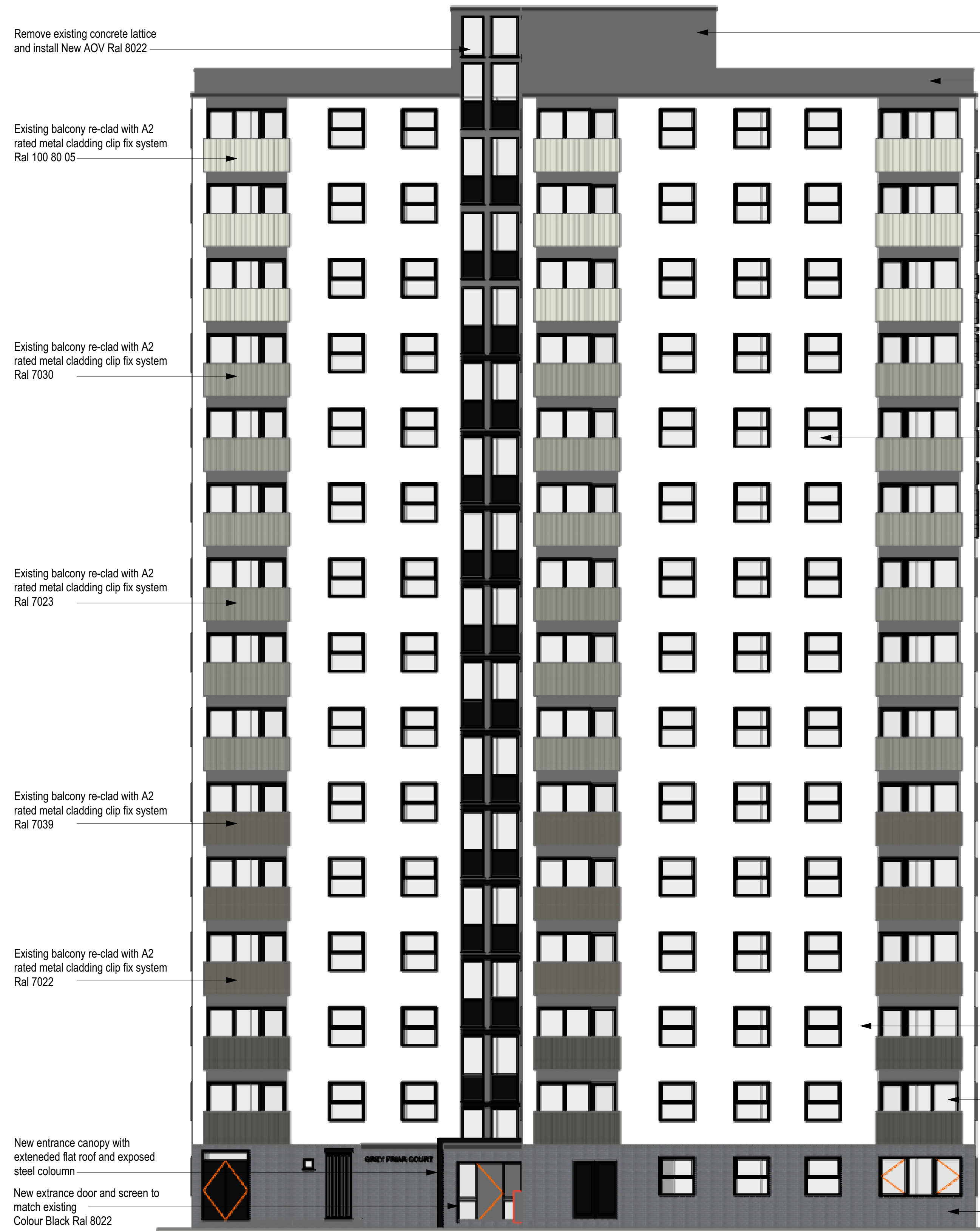
GREY FRIAR COURT FRONT ELEVATION
